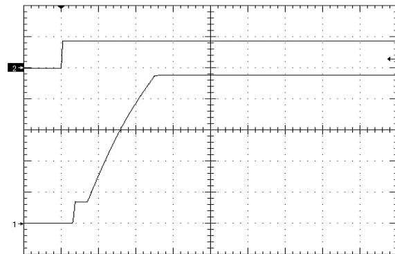
Figure 10. Startup Waveform via Enable Pin, time scale 10mS/div. Vin=Vin_nom, full res. load + 330uF, positive enbl, Ch1=10V/div, Ch2=5V/div
