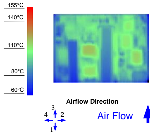
Figure 8. Thermal Image for Airflow Direction 3 (18A output, 55°C ambient, 200 LFM, typical Vin, open frame, unit soldered onto a fixture board)
