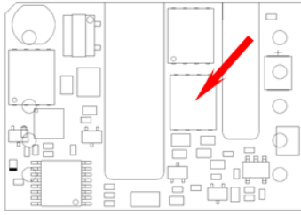
Figure 15. Temperature Monitoring Locations
