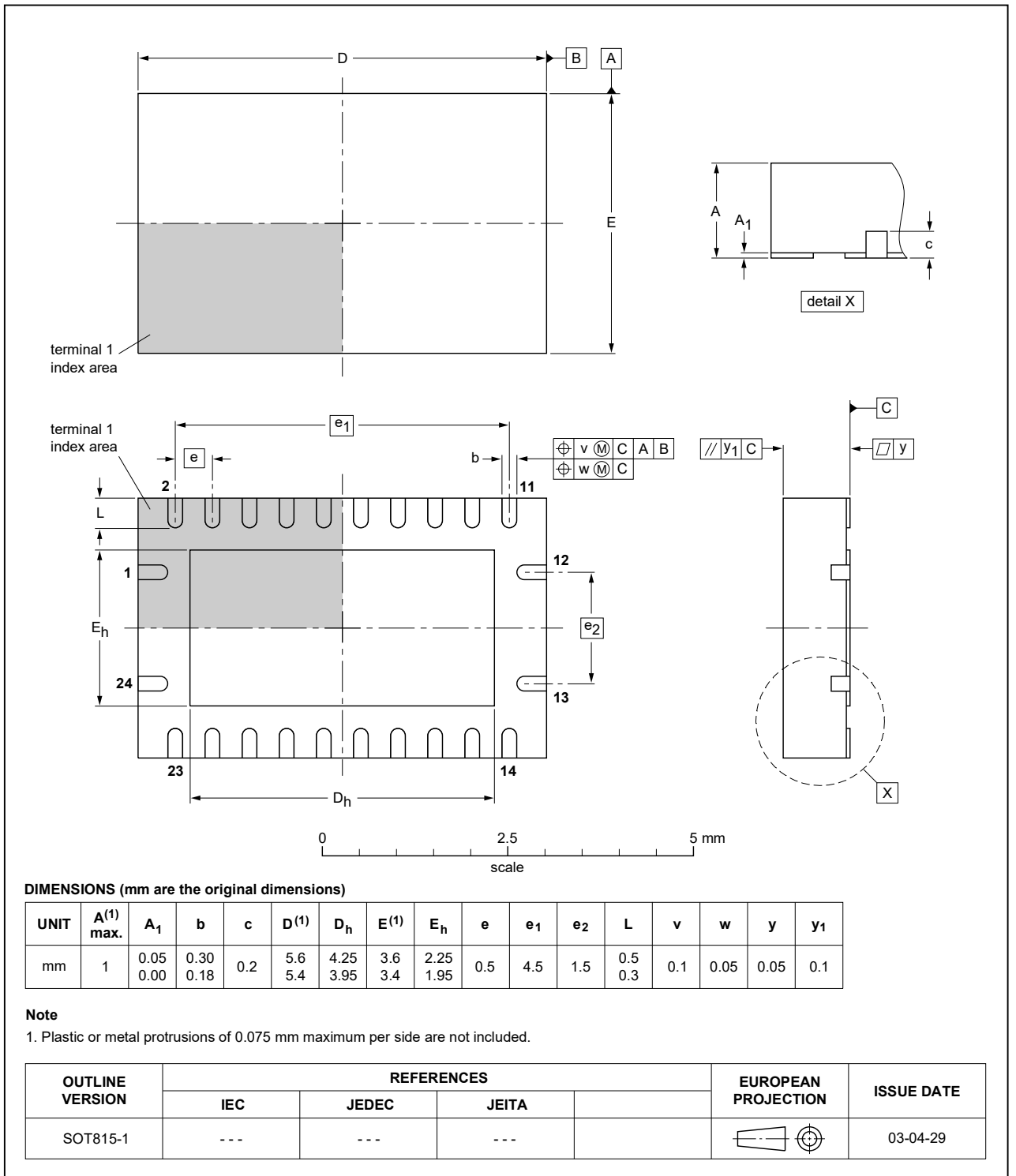
Figure 8. Package outline DHVQFN24
