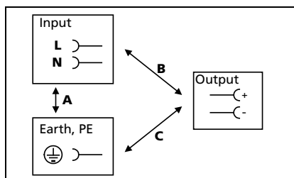
Fig. 17-1 Dielectric strength
