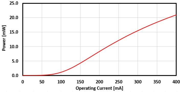
FIG. 7: SLED 3 OUTPUT POWER VS CURRENT
