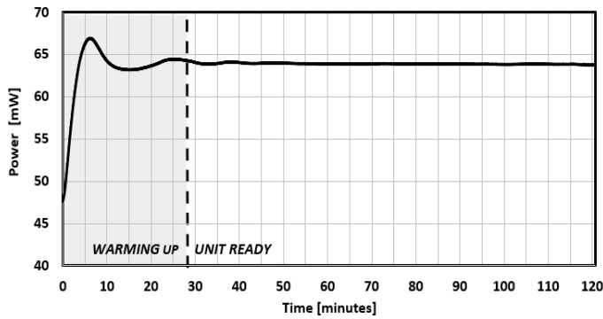
FIG. 9: WARM-UP TIME
