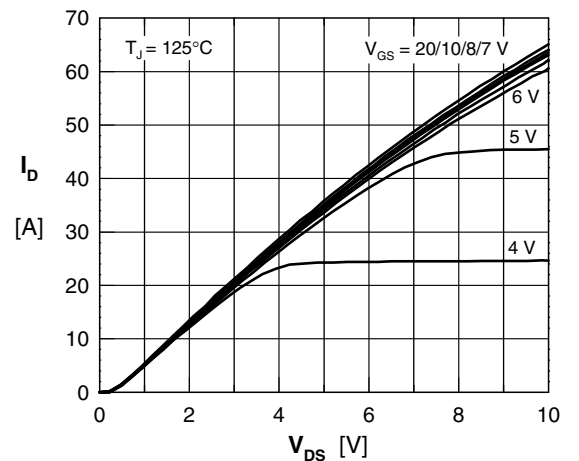
Fig. 4 Typical output characteristic (between pin 5 and pin 2)
