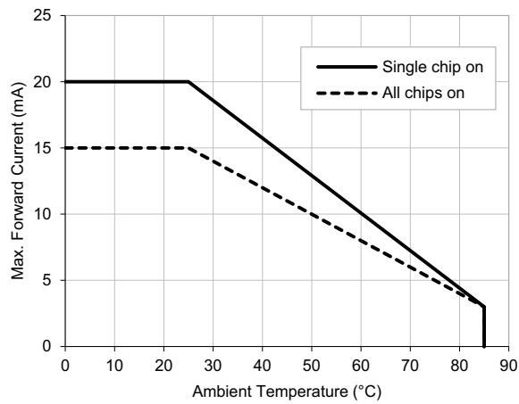
Figure 9: Maximum Forward Current vs. Ambient Temperature
