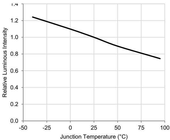
Figure 5: Relative Intensity vs. Junction Temperature
