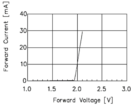
Fig 1. Forward Current vs. Forward Voltage(One chip)
