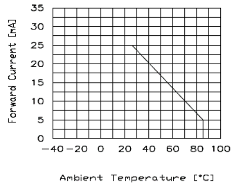
Fig 6. Maximum allowable DC current per segment vs. A function of ambient temperature(One chip)
