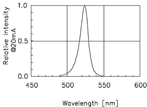
Fig 5. Relative Intensity vs. Wavelength(One chip)
