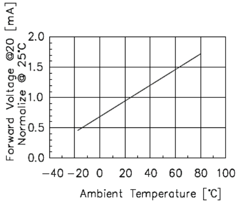
Fig 3. Forward Voltage vs. Temperature(One chip)
