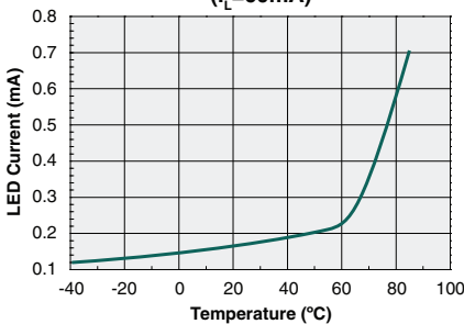
Typical I_F for Switch Operation ( I_L=60mA )
