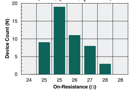
Typical On-Resistance Distribution (N=50, I_F=0mA , I_L=100mA )
