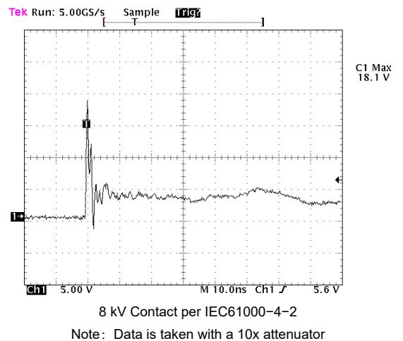
Fig. 6 - ESD Clamping Voltage
