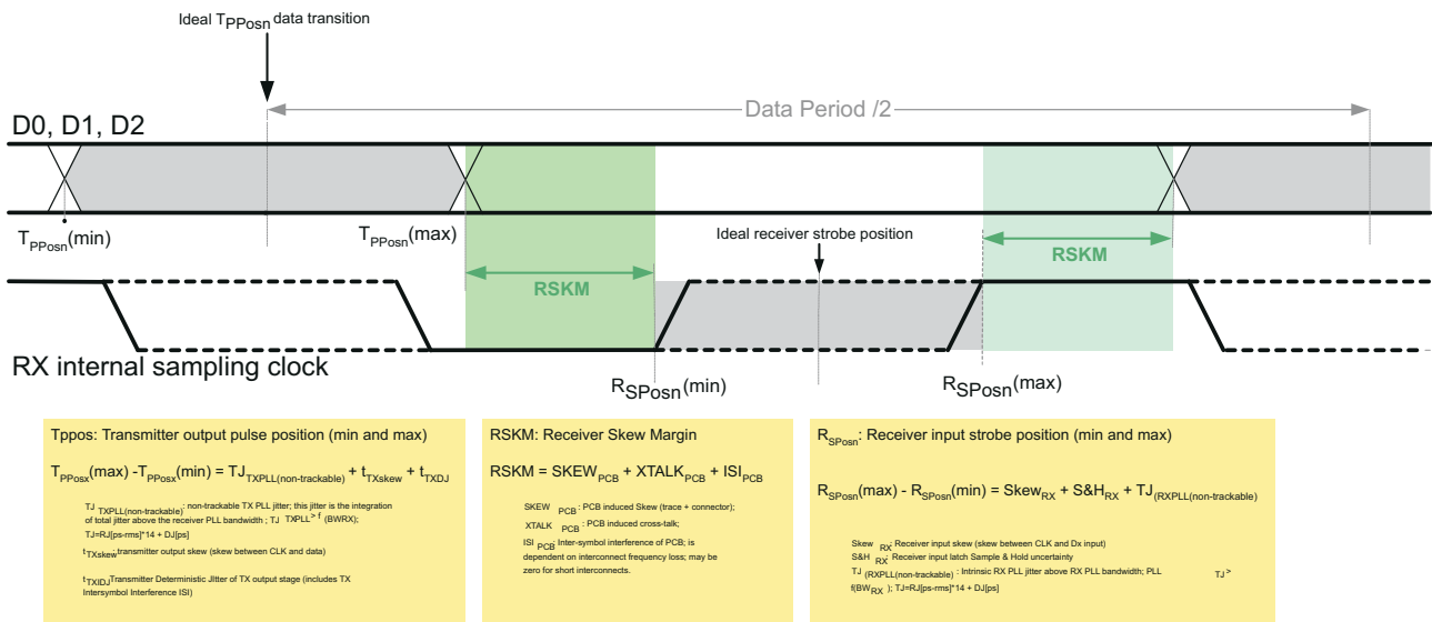
Figure 9-2. Jitter Budget
