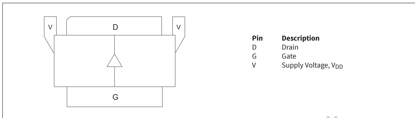
Lead connections for PXFE211507FC
