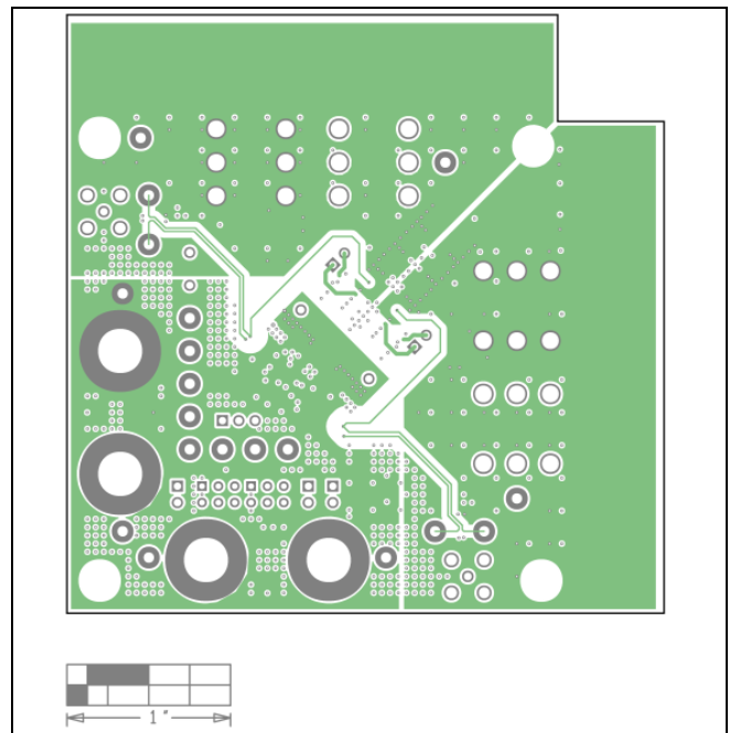
MAX20808 EV Kit PCB Layout—Layer 3
