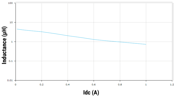
L0806C4R7MDMIT
