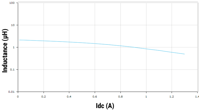
L1008C2R2MDMIT
