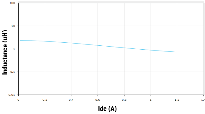
L0806C2R2MDMIT
