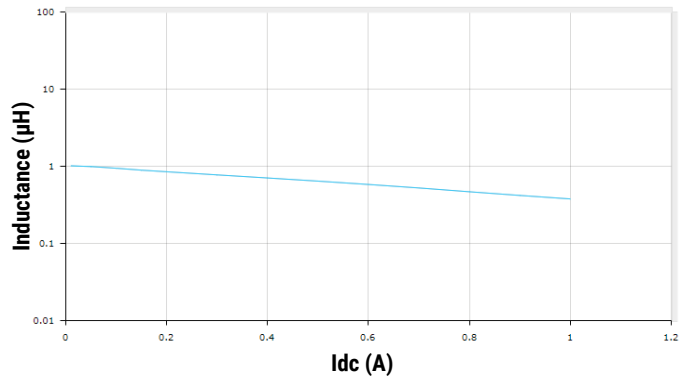
L0603C1R0MDMIT
