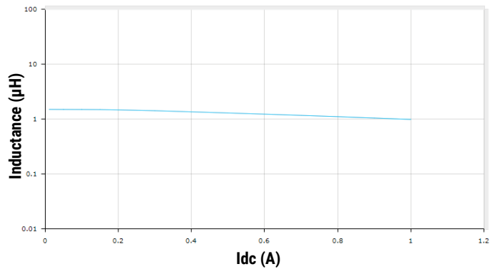
L0805C1R5MDMIT
