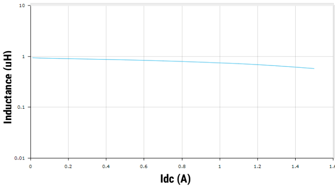
L1008C1R0MDMIT
