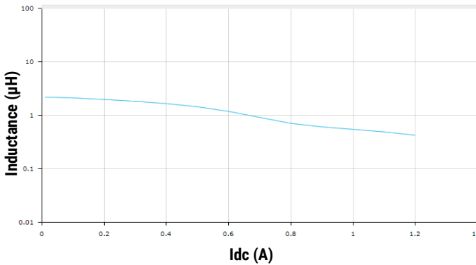
L1008L2R2MDMIT
