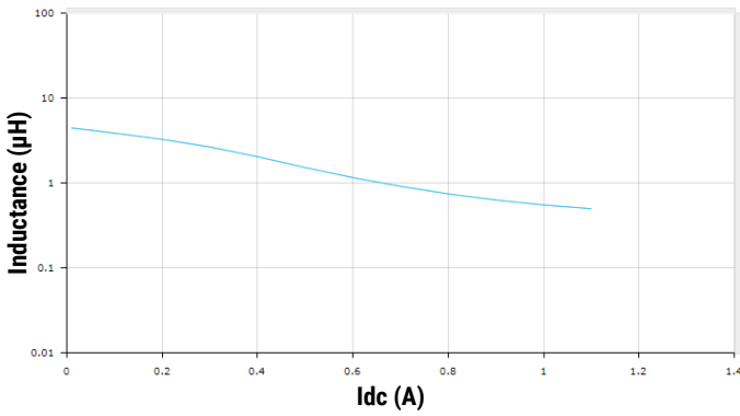
L1008C4R7MDMIT
