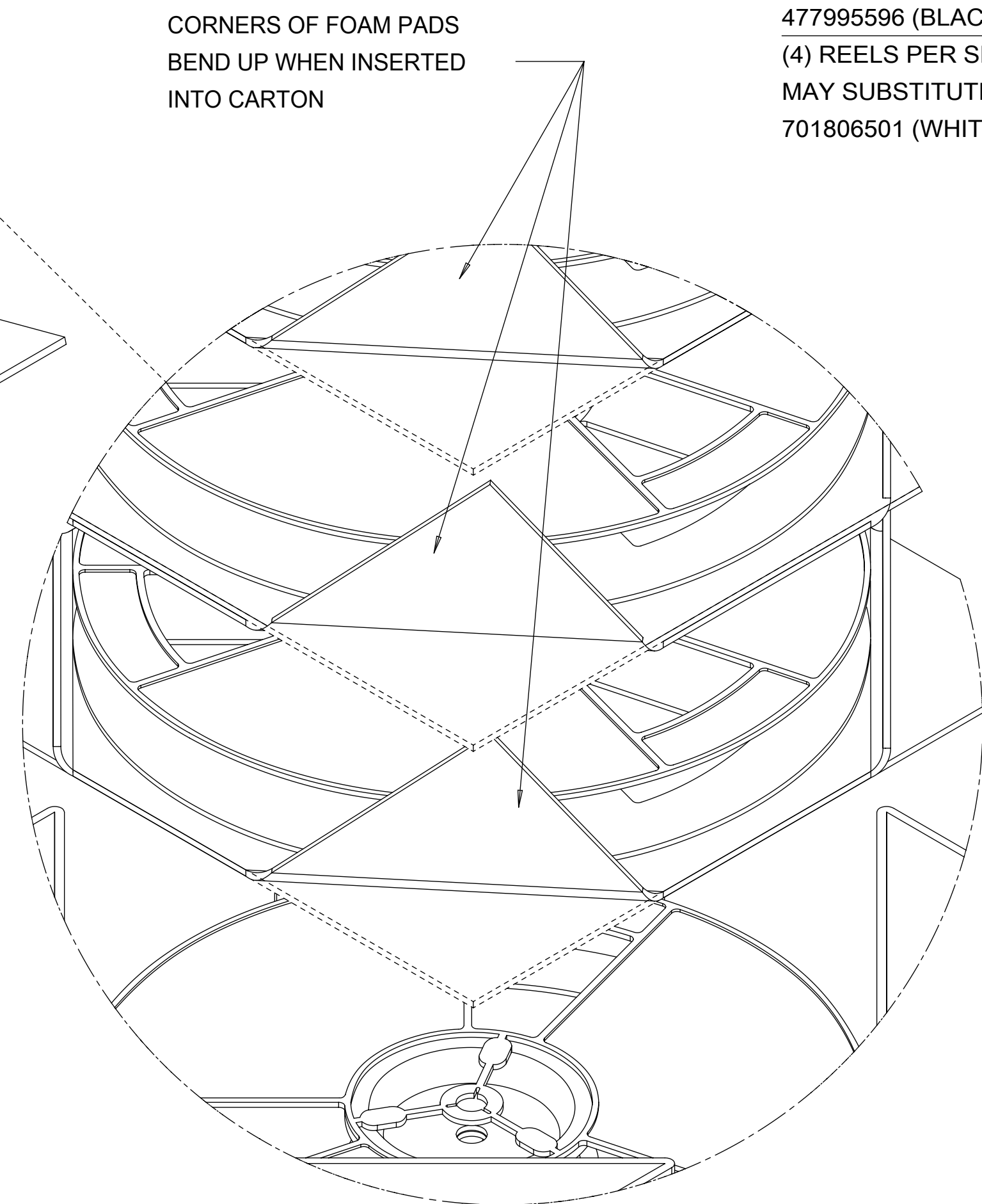
VIEW OF LOADED TAPE AND REEL
