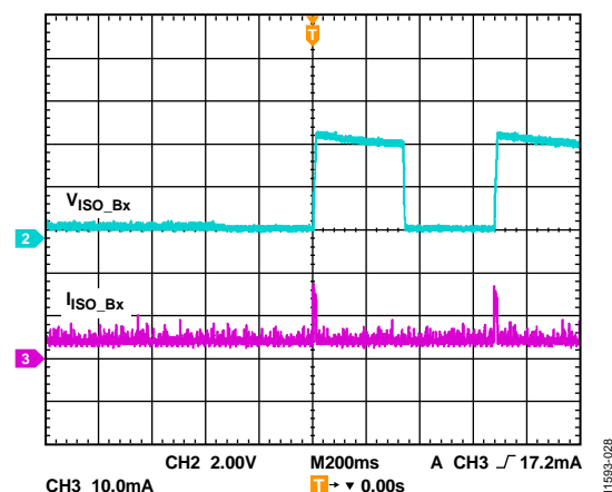
Figure 25. Battery Detection Waveform, V_{SYS}[2:0] = 000 (Binary) = 4.3 V, No Battery
