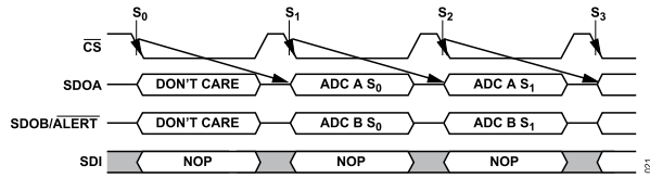
Figure 43. Reading Conversion Results for 2-Wire Mode
