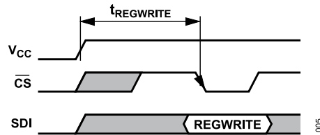
Figure 5. Power-Up Time to Register Read Write Access
