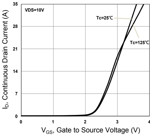
Figure 9. Transfer Characteristics
