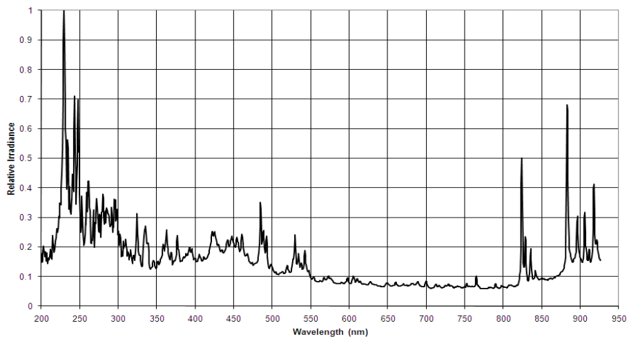
RSL-3100 Spectral Distribution
