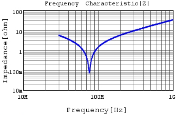
RCE5C2E821J1M1H03A |Z| DC0V, 25degC
