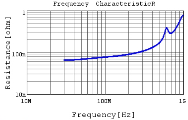
RCE5C2E821J1M1H03A R DC0V, 25degC
