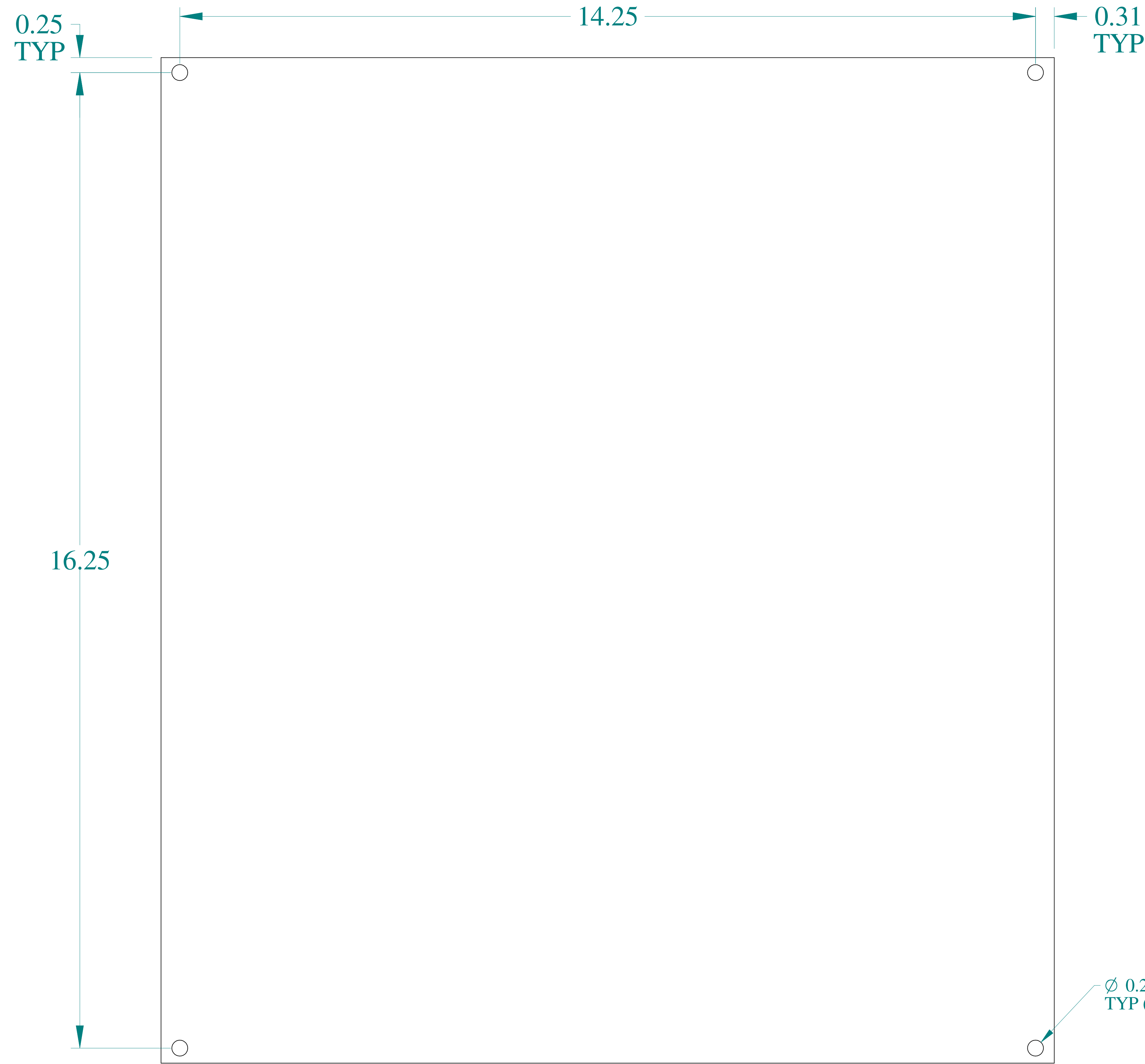
FRONT VIEW
