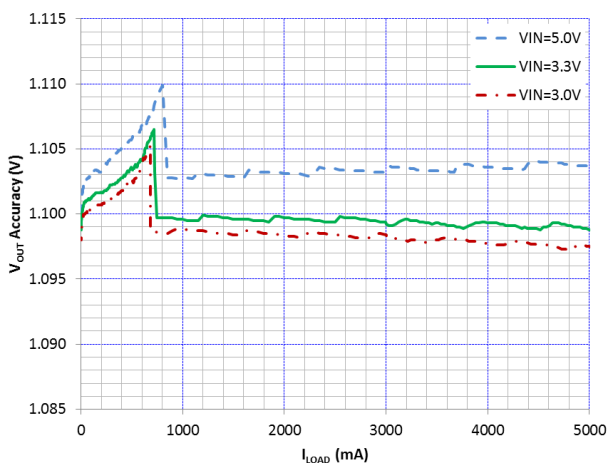
Figure 21. V_{OUT} Accuracy vs I_{LOAD} and V_{IN} V_{OUT} = 1.10\text{ V}
