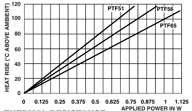
THERMAL RESISTANCE
