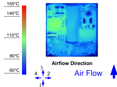
Figure 10. Thermal Image for Airflow Direction 3 (3A output, 55°C ambient, 200 LFM, typical V_{in} , open frame unit)
