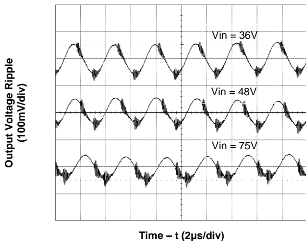
Figure 5. Output Voltage Ripple at Full Load (tested with 8x47µF ceramic output capacitors)
