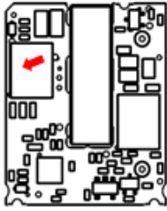
Figure 17. Temperature Monitoring Locations
