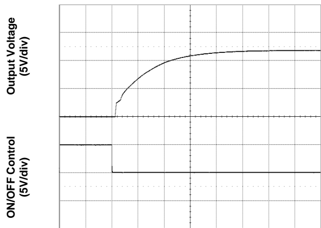
Figure 6. Start-Up from Enable Control (typical Vin, full load, no external output capacitor)
