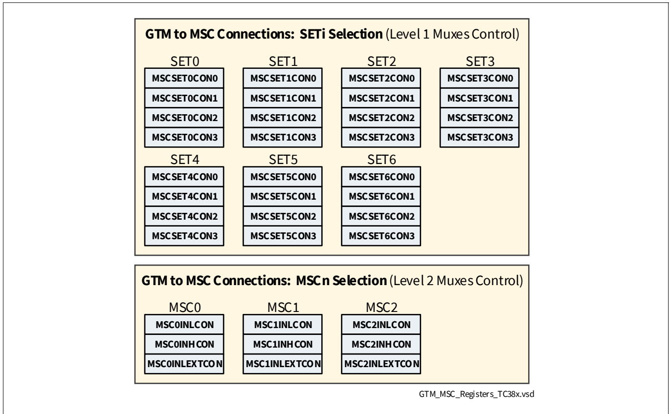
Figure 13 GTM to MSC Connections Registers Overview
