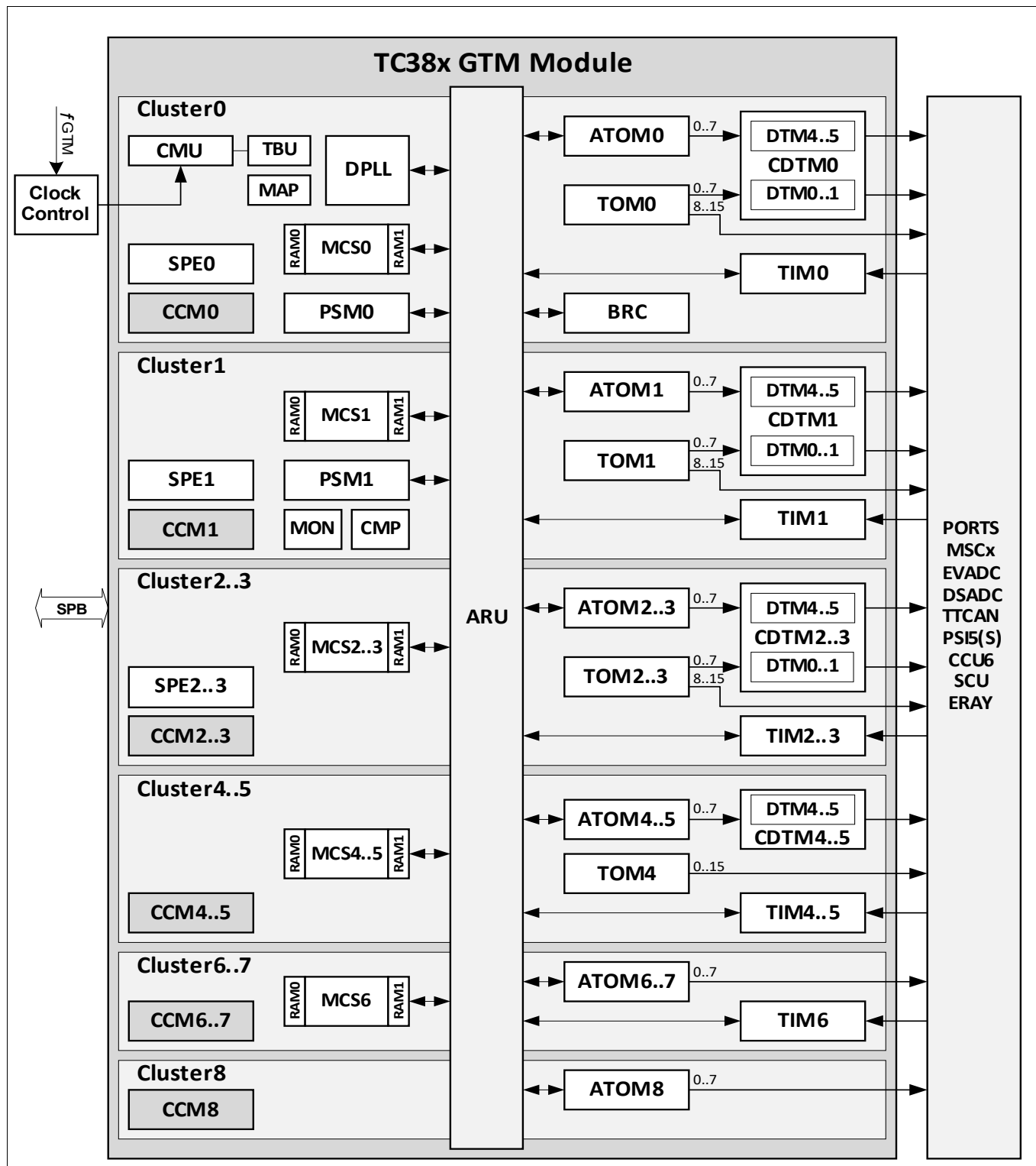
Figure 5 GTM IP Block Diagram (TC38x)
