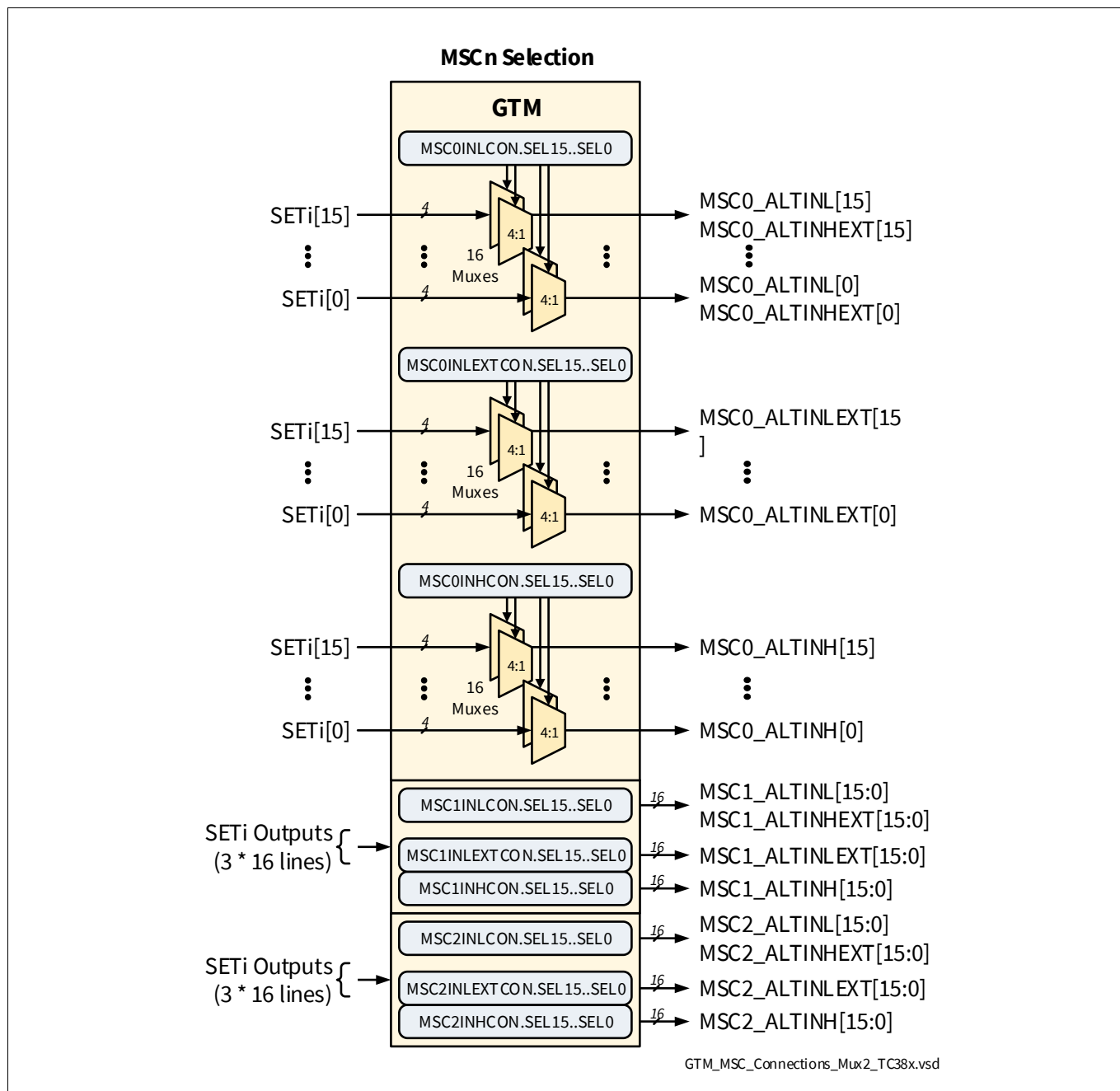
Figure 15 GTM to MSC Connections, 2nd Level Muxes Overview
