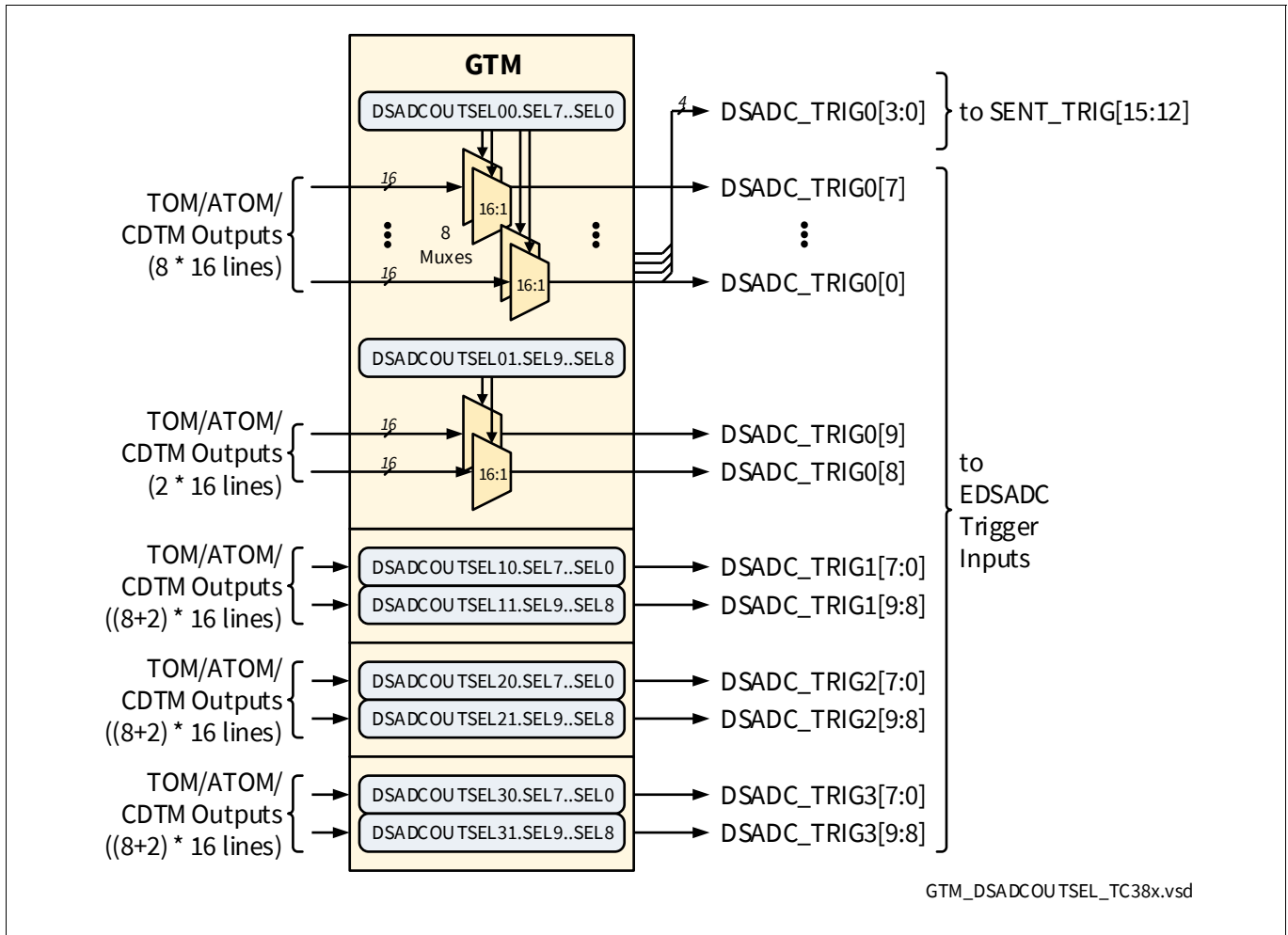
Figure 18 GTM to EDSADC Connections Overview
