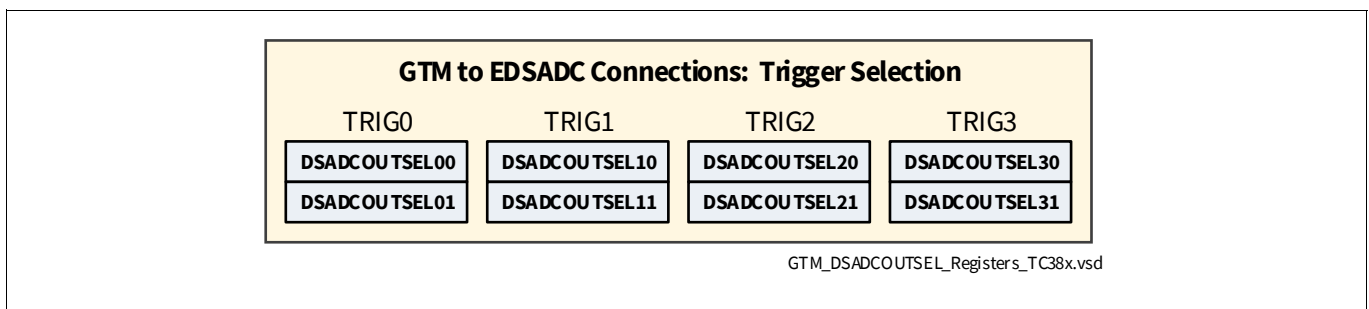
Figure 19 GTM to EDSADC Connections Registers Overview
