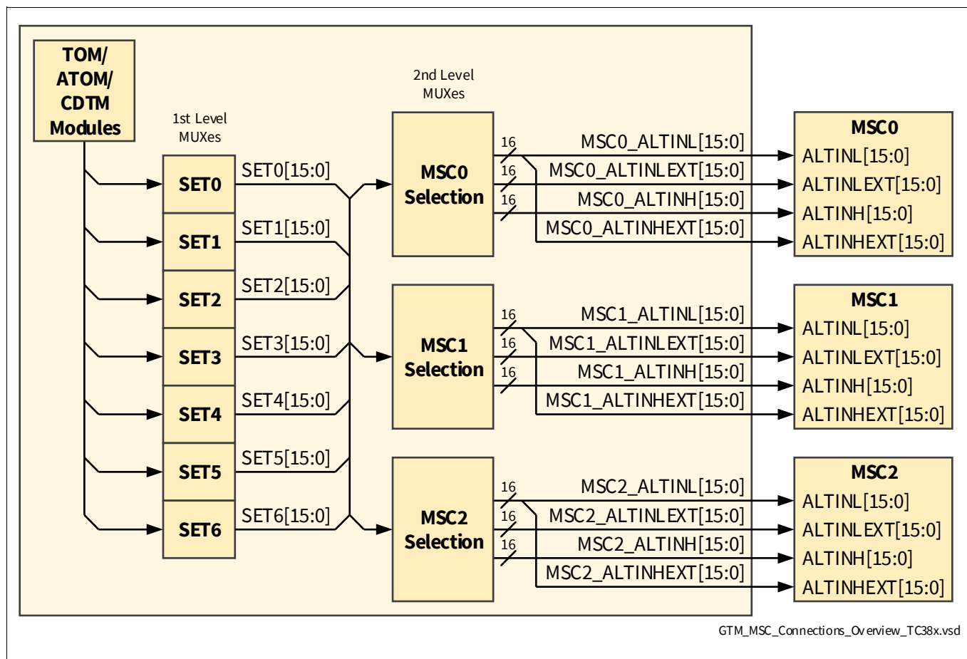
Figure 12 GTM to MSC Connections Overview
