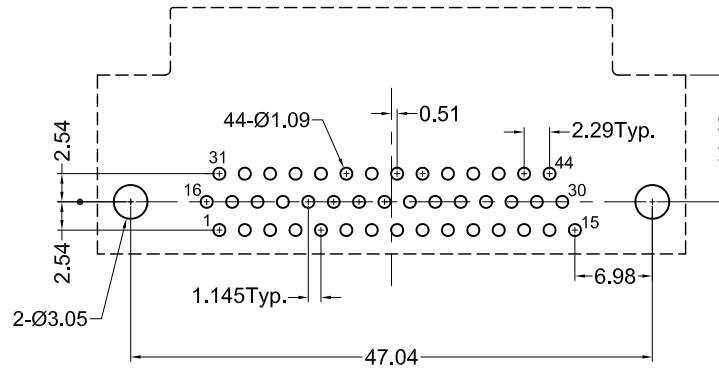
Recommended PCB Layout (Bottom View)
