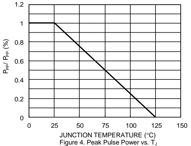
Figure 4. Peak Pulse Power vs. T_J
