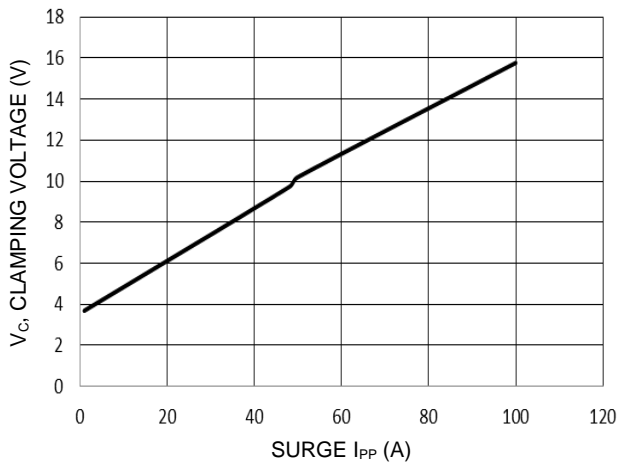
Figure 7. Clamping Voltage Characteristics ( t_p = 8/20\mu s )
