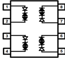
Device Schematic
