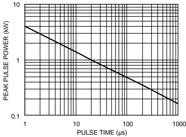
Figure 3. Power Dissipation vs. Pulse Time
