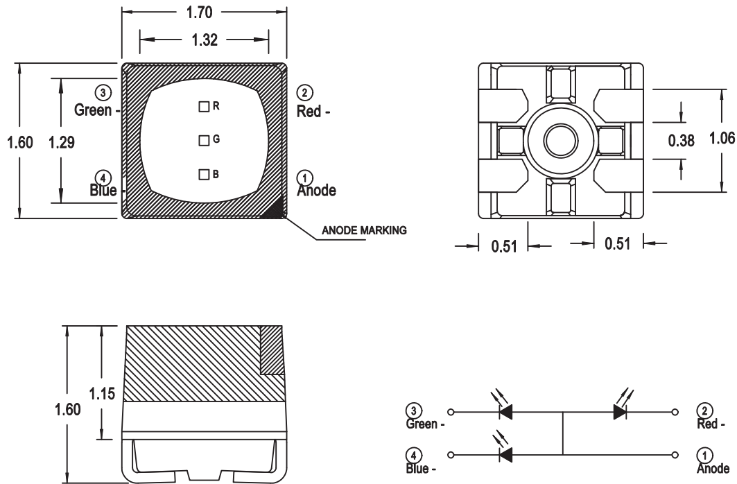
Figure 1: Package Drawing
