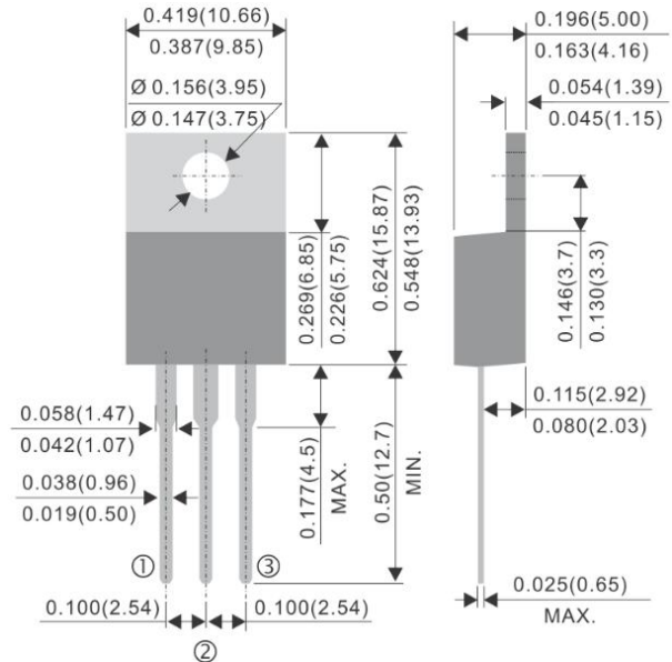
TO-220AB Dimension
