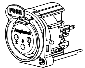
3D VIEW (1:1)
