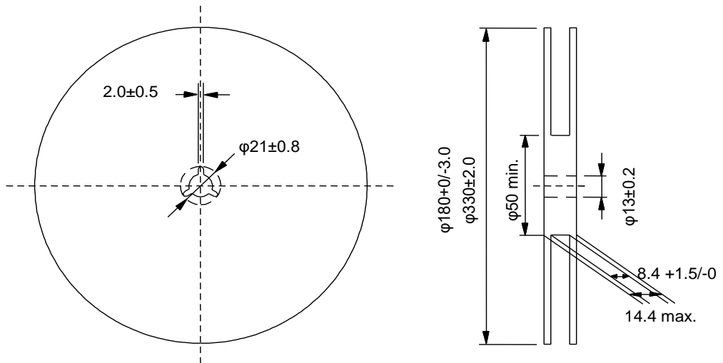
Fig.3 Taping Diagram
