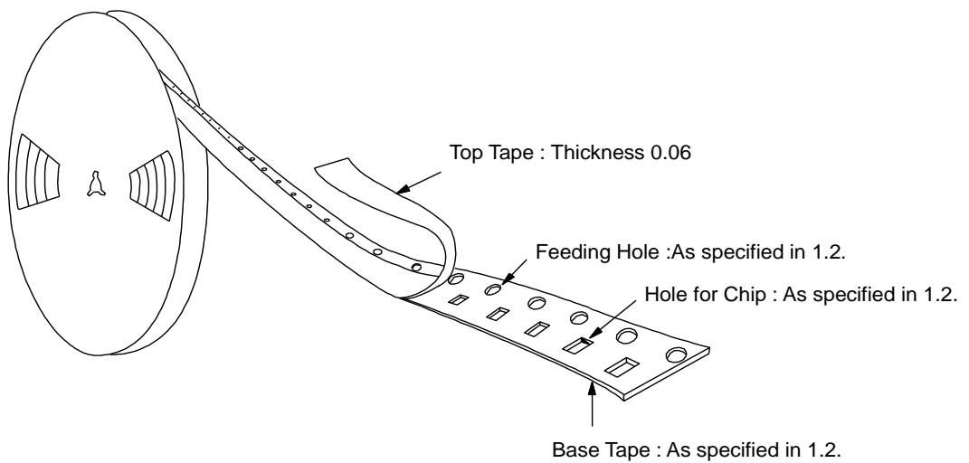
Fig.3 Taping Diagram
