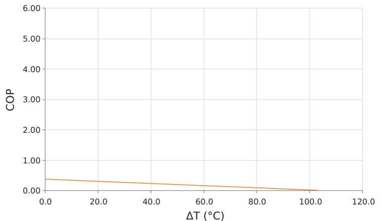
Coefficient of Performance (COP = Qc/Pin) Thot = 27 °C | Current = 6.4 Amps
