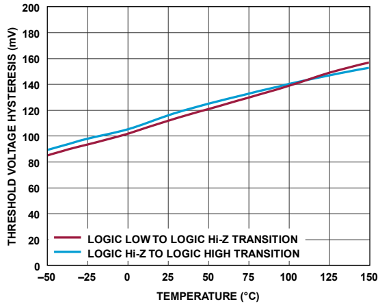
Figure 28. V O0 , V O1 , V O2 and MARG Pin Hysteresis
