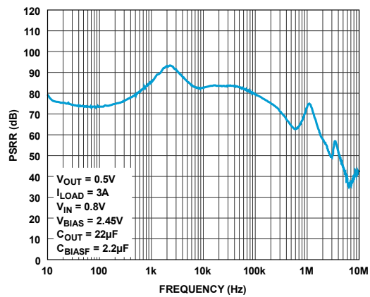
Figure 53. BIAS Pin PSRR
