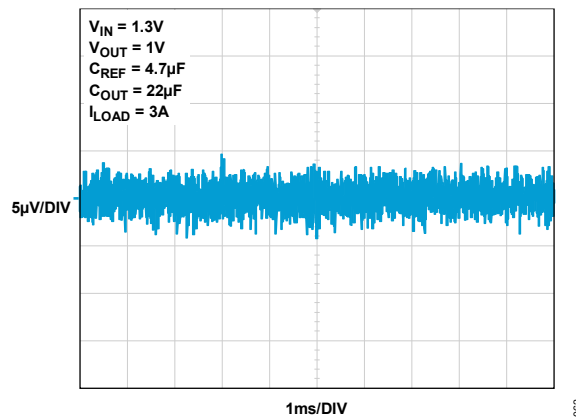
Figure 62. Output Noise (10Hz to 100kHz)
