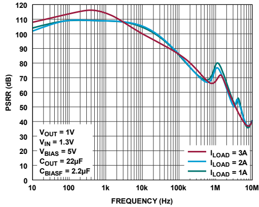
Figure 52. BIAS Pin PSRR
