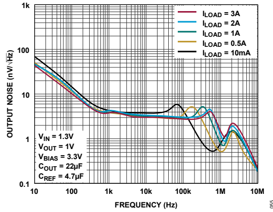
Figure 55. Noise Spectral Density
