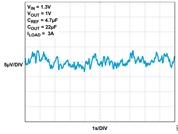
Figure 63. Output Noise (0.1Hz to 10Hz)
