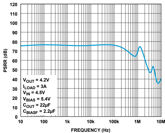
Figure 54. BIAS Pin PSRR
