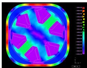
Magnetic Field
