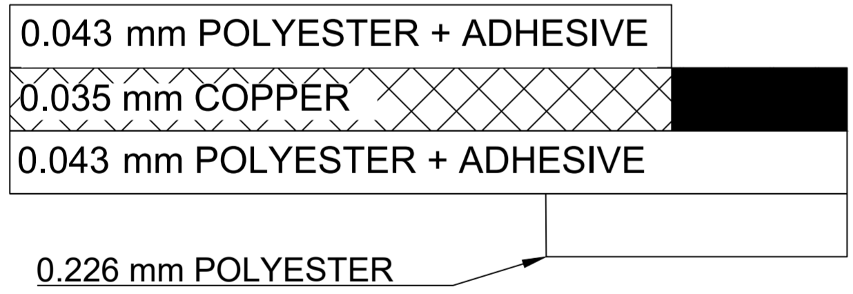
CROSS-SECTION
