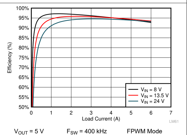
Figure 9-10. LMQ61460 Efficiency
