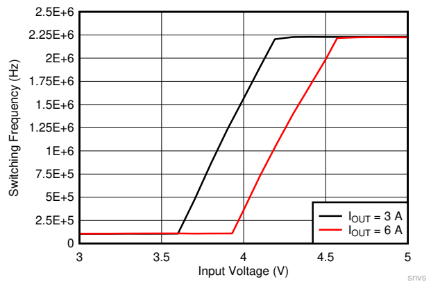
Figure 9-24. LMQ61460 Dropout Curve
