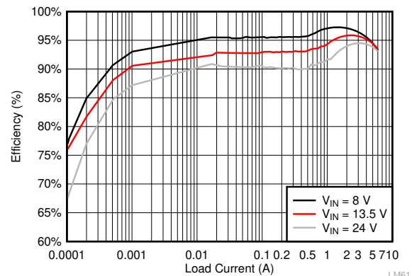
Efficiency: V OUT = 5 V, F SW = 400 kHz
