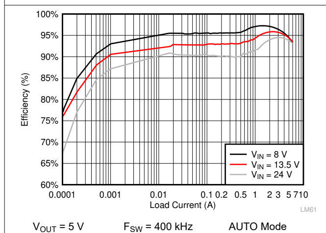
Figure 9-9. LMQ61460 Efficiency
