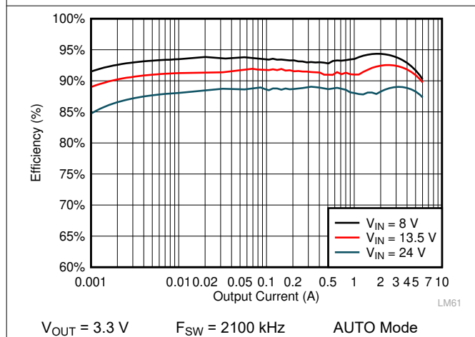
Figure 9-5. LMQ61460 Efficiency
