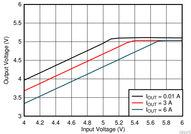
Figure 9-23. LMQ61460 Dropout Curve
