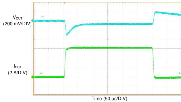
Figure 9-39. LMQ61460 Load Transient
