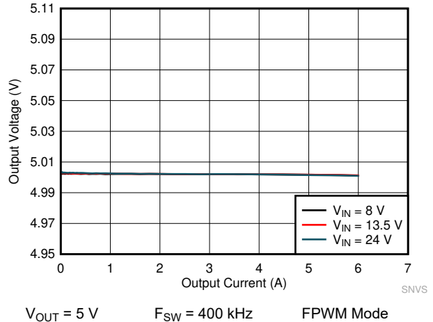
Figure 9-18. LMQ61460 Load and Line Regulation
