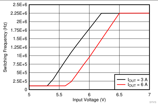
Figure 9-26. LMQ61460 Frequency Dropout Curve
