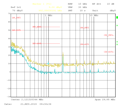
Figure 9-52. Radiated EMI Log Horizontal versus CISPR25 Limits
