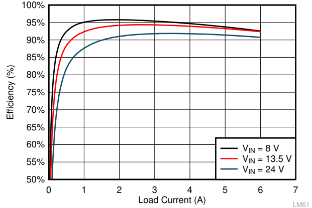
Figure 9-12. LMQ61460 Efficiency
