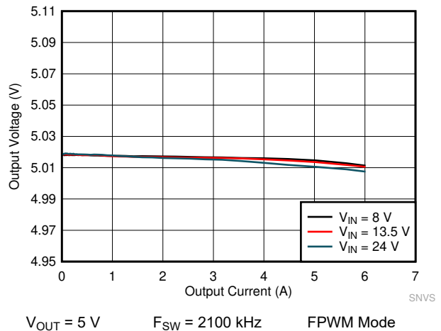
Figure 9-20. LMQ61460 Load and Line Regulation
