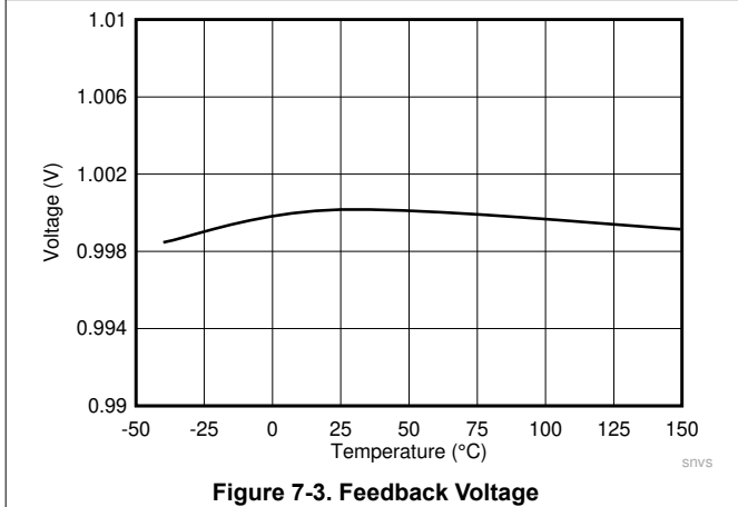
Figure 7-3. Feedback Voltage
