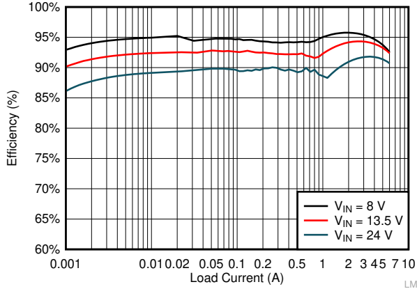
Figure 9-11. LMQ61460 Efficiency
