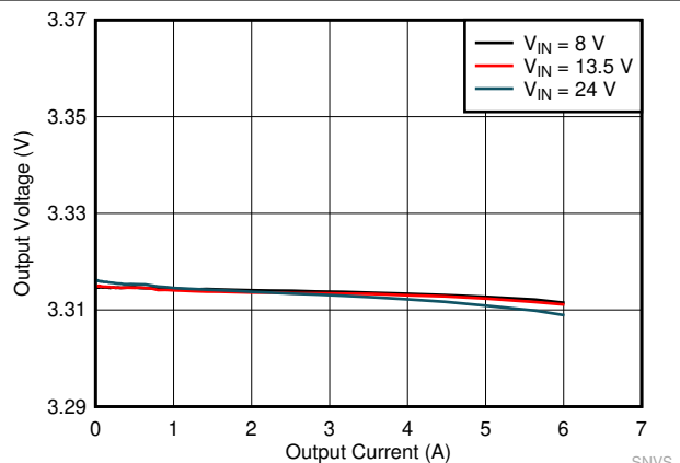
Figure 9-14. LMQ61460 Load and Line Regulation
