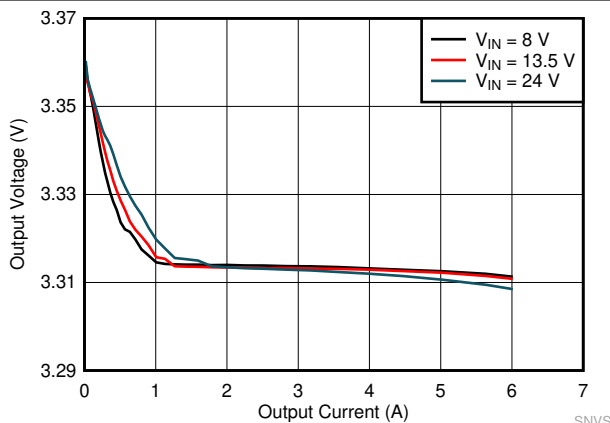
Figure 9-13. LMQ61460 Load and Line Regulation
