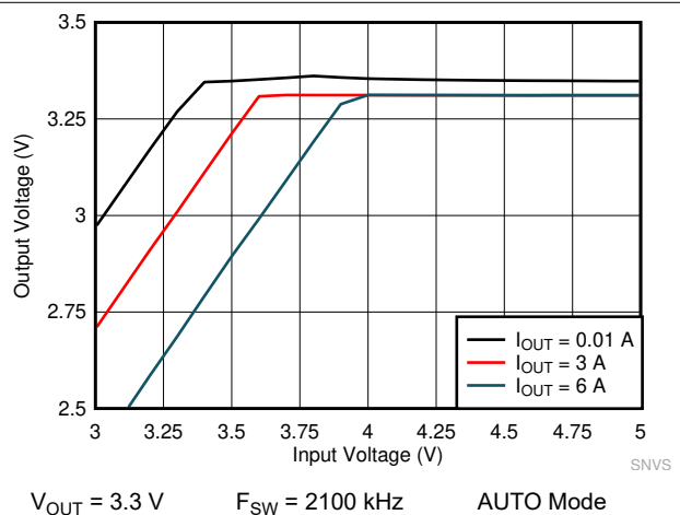
Figure 9-22. LMQ61460 Dropout Curve
