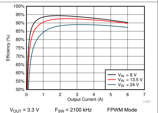
Figure 9-6. LMQ61460 Efficiency
