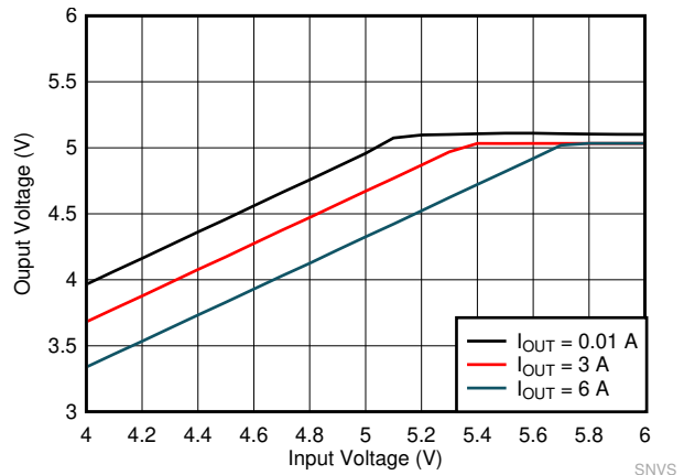
Figure 9-24. LMQ61460 Dropout Curve
