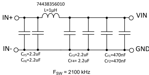
Figure 9-61. Recommended Input EMI Filter
