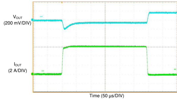
Figure 9-40. LMQ61460 Load Transient
