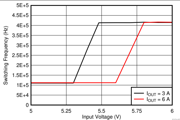
Figure 9-25. LMQ61460 Frequency Dropout Curve
