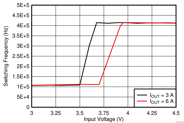
Figure 9-23. LMQ61460 Dropout Curve
