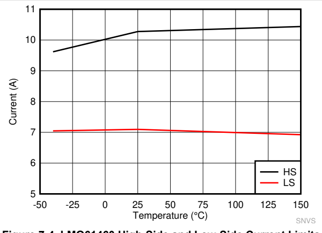
Figure 7-4. LMQ61460 High-Side and Low-Side Current Limits
