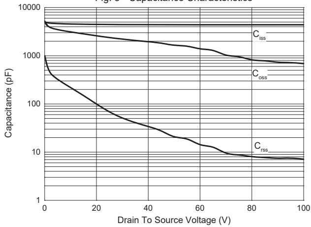
Fig. 3 - Capacitance Characteristics
