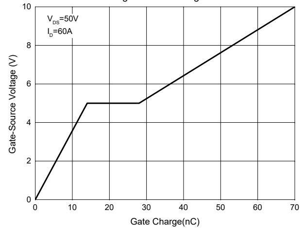
Fig. 4 - Gate Charge
