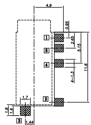
RECOMMENDED PCB LAYOUT (COPPER SIDE)
