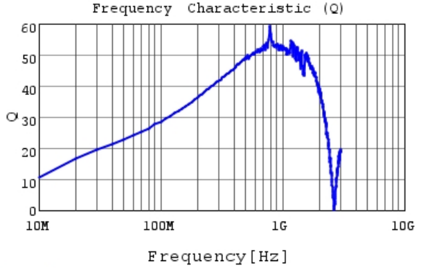
LQW15AW68NJ80 Q
