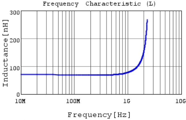
LQW15AW68NJ80 L
