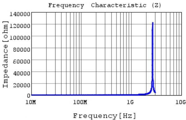
LQW15AW68NJ80 |Z|
