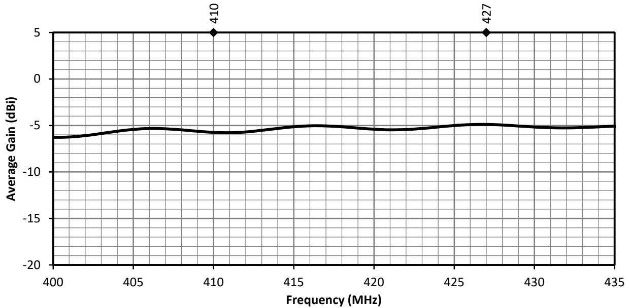
Figure 15. ANT-418-WRT Antenna Average Gain, at Center of Ground Plane
