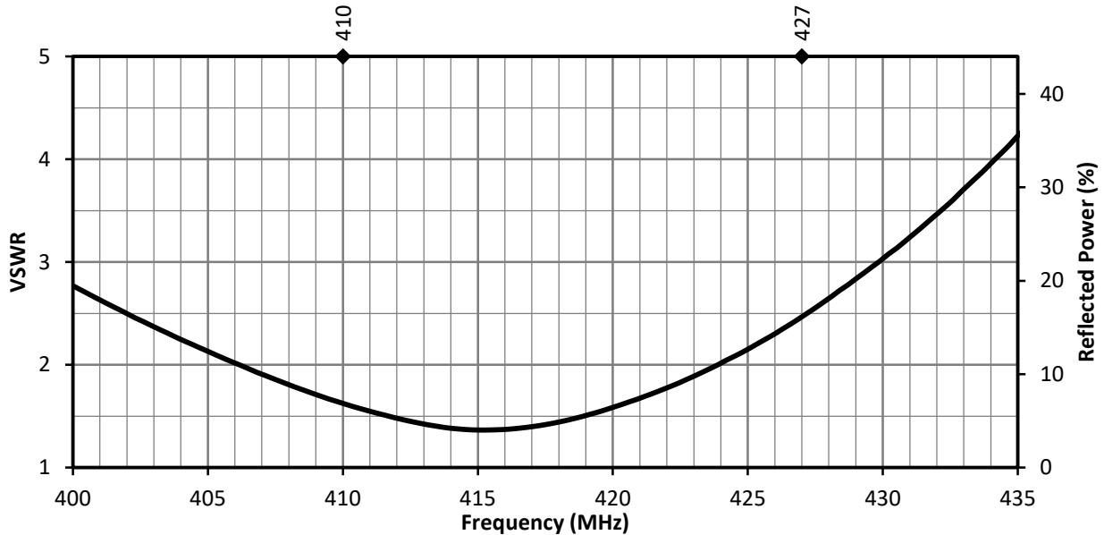
Figure 12. ANT-418-WRT VSWR, at Center of Ground Plane
