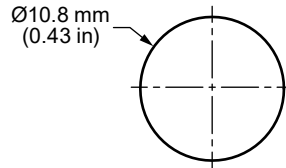
Figure 2. ANT-418-WRT Series Antenna Recommended Enclosure Mounting Dimensions
