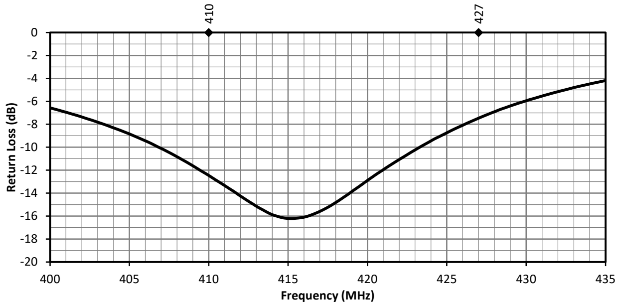
Figure 13. ANT-418-WRT Return Loss, at Center of Ground Plane
