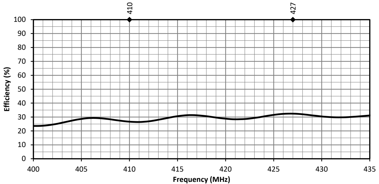
Figure 16. ANT-418-WRT Antenna Radiation Efficiency, at Center of Ground Plane
