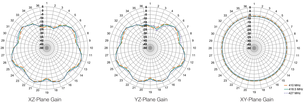
Figure 17. ANT-418-WRT Radiation Patterns, Center of Ground Plane
