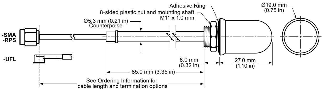
Figure 1. ANT-418-WRT Antenna Dimensions
