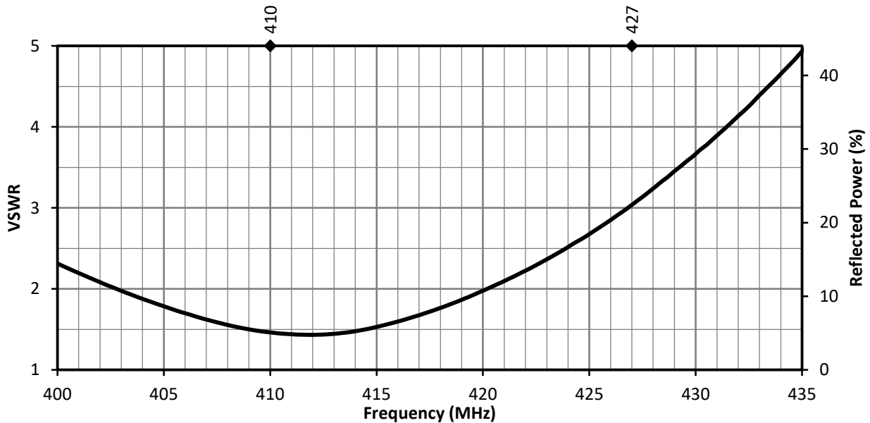
Figure 5. ANT-418-WRT VSWR, Free Space
