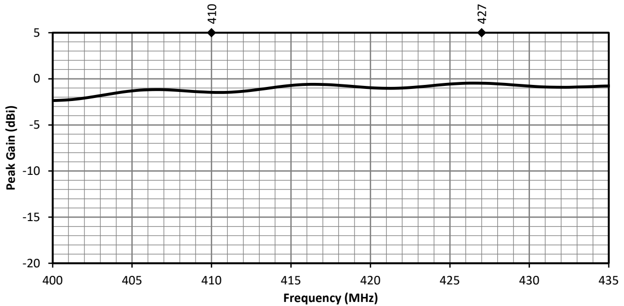
Figure 14. ANT-418-WRT Peak Gain, at Center of Ground Plane
