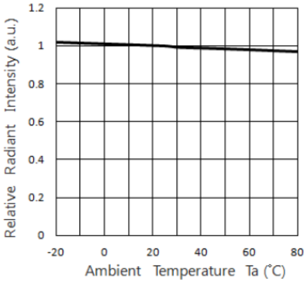
1 Relative Radiant Intensity & Ambient Temperature
