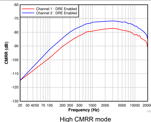
Figure 7-27. Common-Mode Rejection Ratio vs Ripple Frequency With 100\text{-mV}_{PP} Amplitude and DRE Enabled
