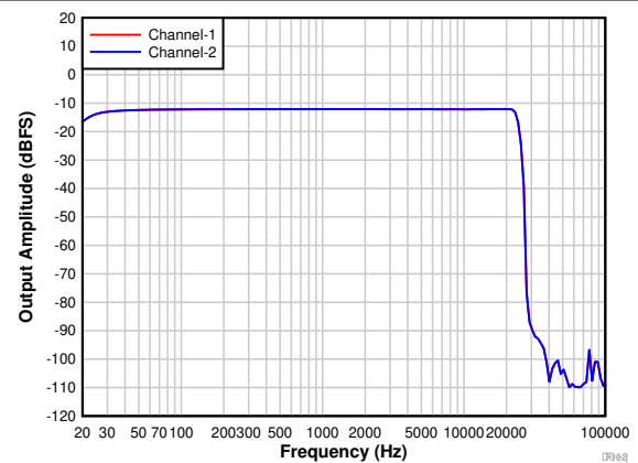
Figure 7-15. Frequency Response With a -12-dBr Input
