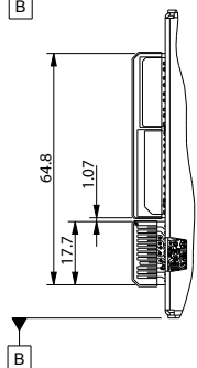
DETAIL A (1:1)
