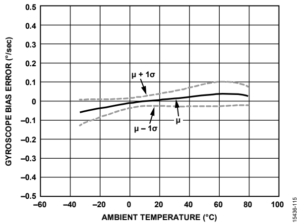
Figure 15. ADIS16475-1 Gyroscopic Bias Error vs. Ambient Temperature
