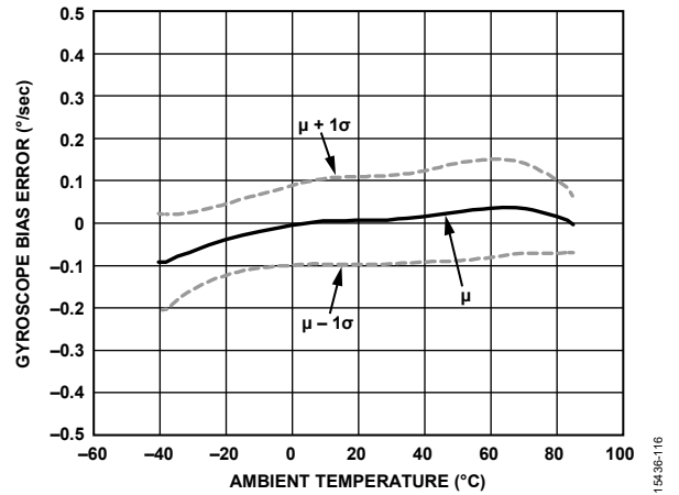
Figure 16. ADIS16475-2 Gyroscopic Bias Error vs. Ambient Temperature
