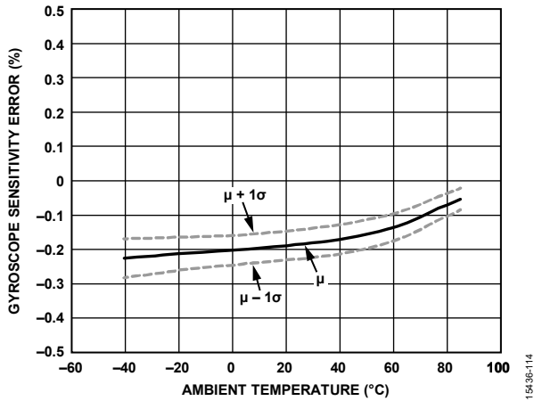
Figure 14. ADIS16475-3 Gyroscopic Sensitivity Error vs. Ambient Temperature
