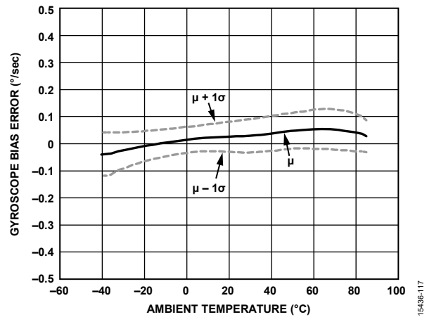
Figure 17. ADIS16475-3 Gyroscopic Bias Error vs. Ambient Temperature
