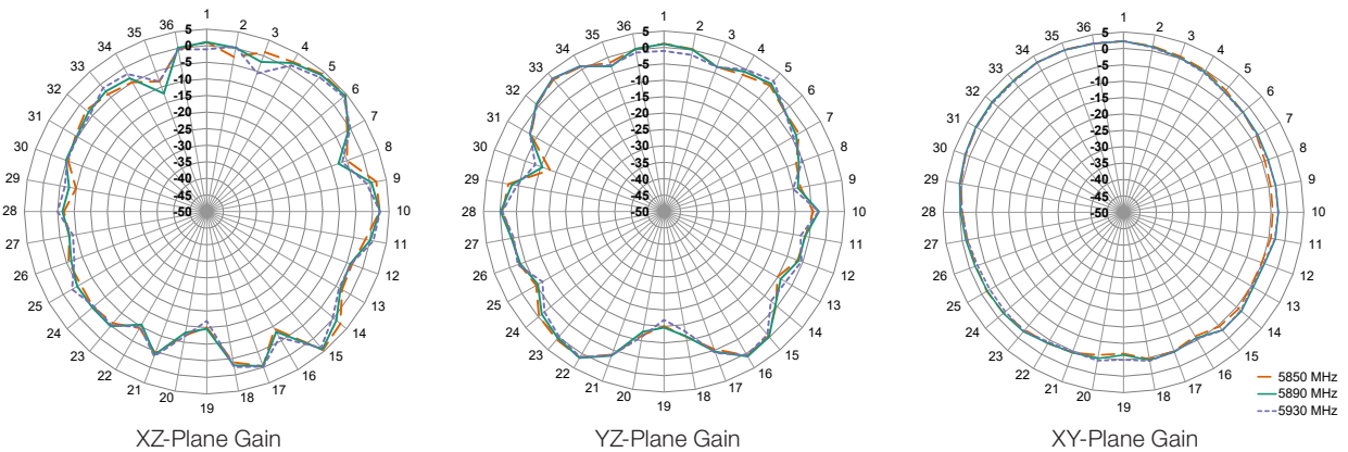
Figure 9. Radiation Patterns for ANT-V2X-IPW1-NP Antenna, Free Space
