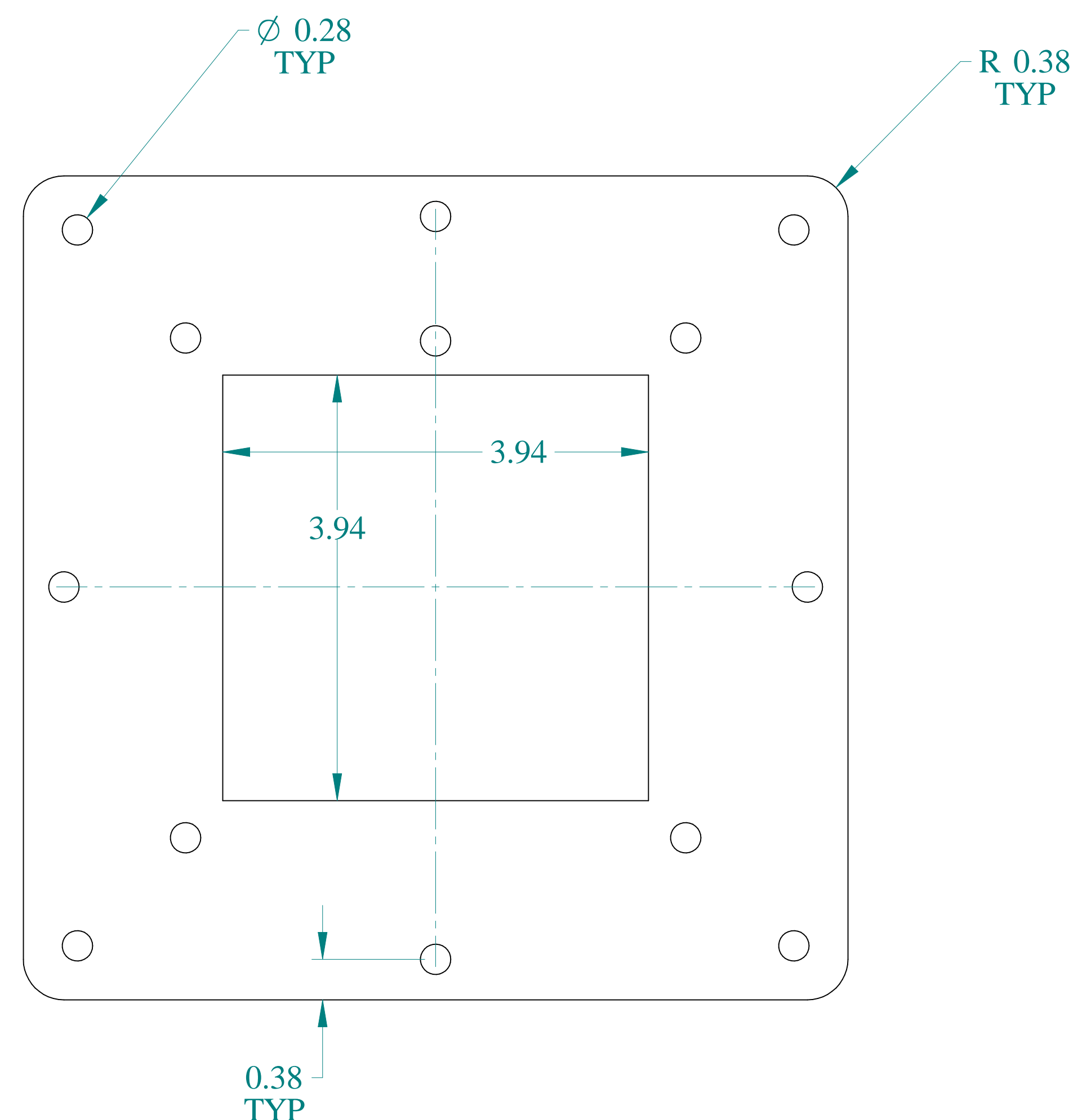
BACK VIEW
