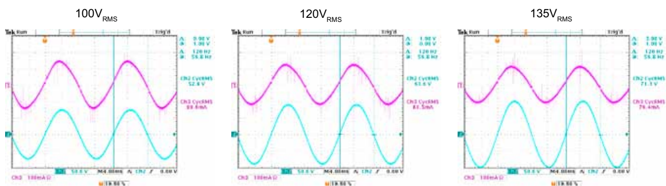
Line Voltage and Current at half load (350mA, 20V)
