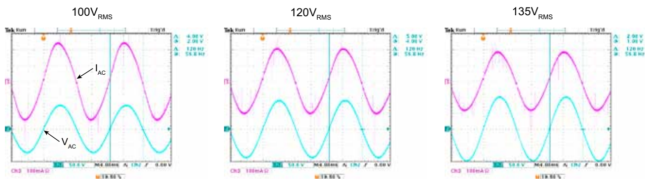
Line Voltage and Current at nominal load (350mA, 40V)
