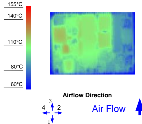
Figure 8. Thermal Image for Airflow Direction 3 (5.8A output, 55°C ambient, 200 LFM, typical Vin, open frame, unit soldered onto a fixture board)
