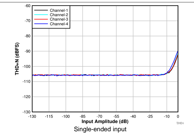
Figure 6. THD+N vs Input Amplitude
