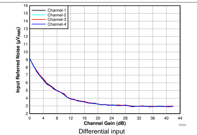
Figure 10. Input-Referred Noise vs Channel Gain
