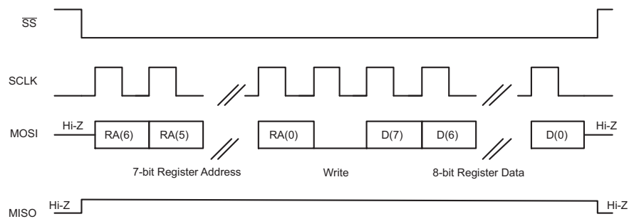
Figure 87. SPI Single-Byte Write Transfer
