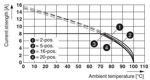
Type: FRONT-MC 1,5/...-STF-3,81 with MCV 1,5/...-GF-3,81 P... THR
